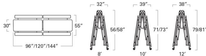
59TV BENCH TABLE - 8', 10', 12' (27"/29" high)
