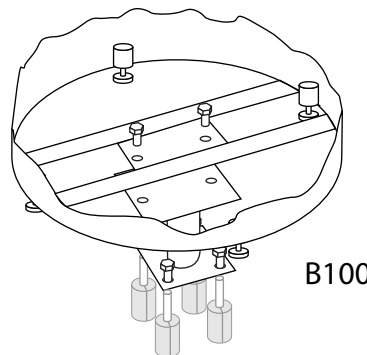
SURFACE MOUNT (2)
