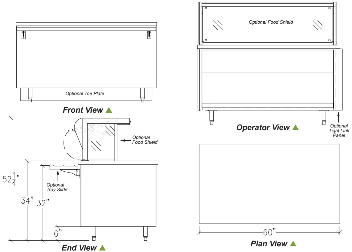
Model PHULS60
