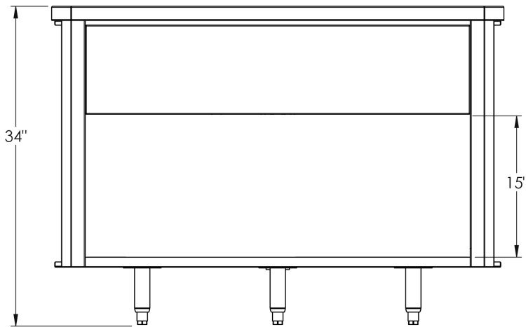
Model PHULS36
