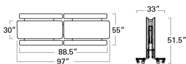
19F BENCH TABLE - 8' (27"/29"/30" high)
