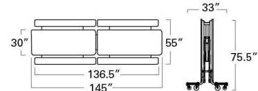
19F BENCH TABLE - 12' (27"/29"/30" high)
