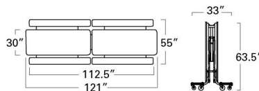
19F BENCH TABLE - 10' (27"/29"/30" high)
