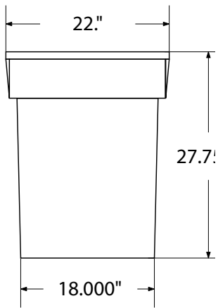
liner
