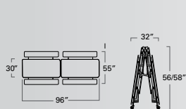
59TV BENCH TABLE - 8' (27"/29" high) 59TV23293008-BNCH 59TV23273008-BNCH
