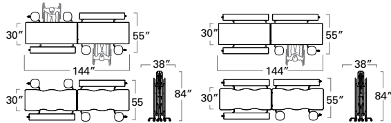
63T 12' BENCH 2WC (30" high) 63T23303012-2BWC 63T23303012W-2BS4 (Wave)
