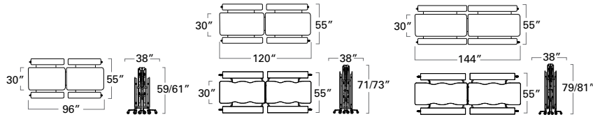
63T 8' BENCH (27"/29" high) 63T23293008 63T23273008
