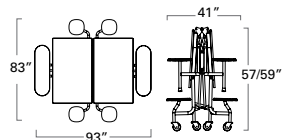
59T SQUARE - 2 BENCH/4 STOOL (27"/29" high) 59T12295263-B2S4 59T12275263-B2S4
