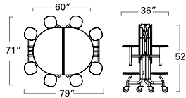
59T ELONGATED - 8 STOOL (27" high only ) 59T122760EL-S8
