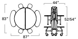
59T ROUND - 2 BENCH, 4 STOOL (27"/29" high) 59T122960RD-B2S4 59T122760RD-B2S4
