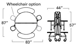
59T ROUND - 2 BENCH/ 2 STOOL/ WC (32" high) 59T123260RD-B2S2
