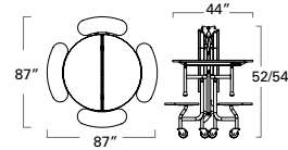
59T ROUND - 4 BENCH (27"/29" high) 59T122960RD-B4 59T122760RD-B4
