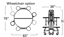
59T ROUND - 6 STOOL/ WC (32" high) 59T123260RD-S6
