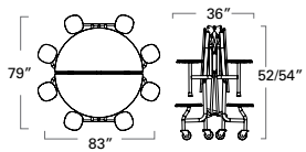
59T ROUND - 8 STOOL (27"/29" high) 59T122960RD-S8 59T122760RD-S8
