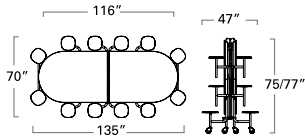
59T ELONGATED - 12 STOOL (27"/29" high) 59T0829120EL-S12 59T0827120EL-S12
